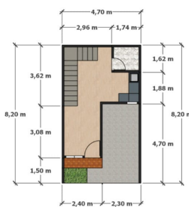
Lantai 1
